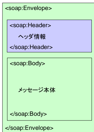
図 3. 1. 1 SOAP Envelope
